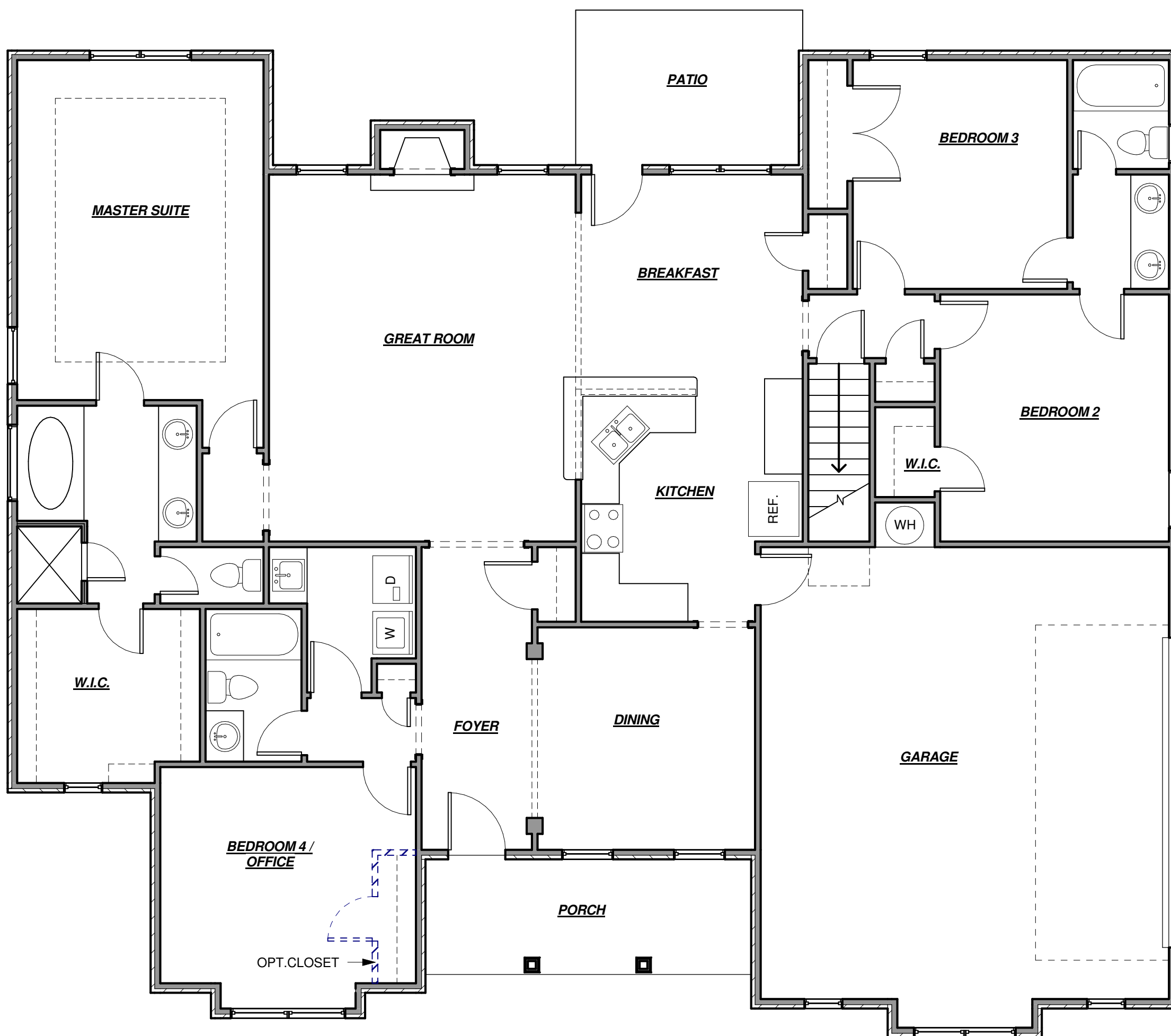
FLOOR PLAN
