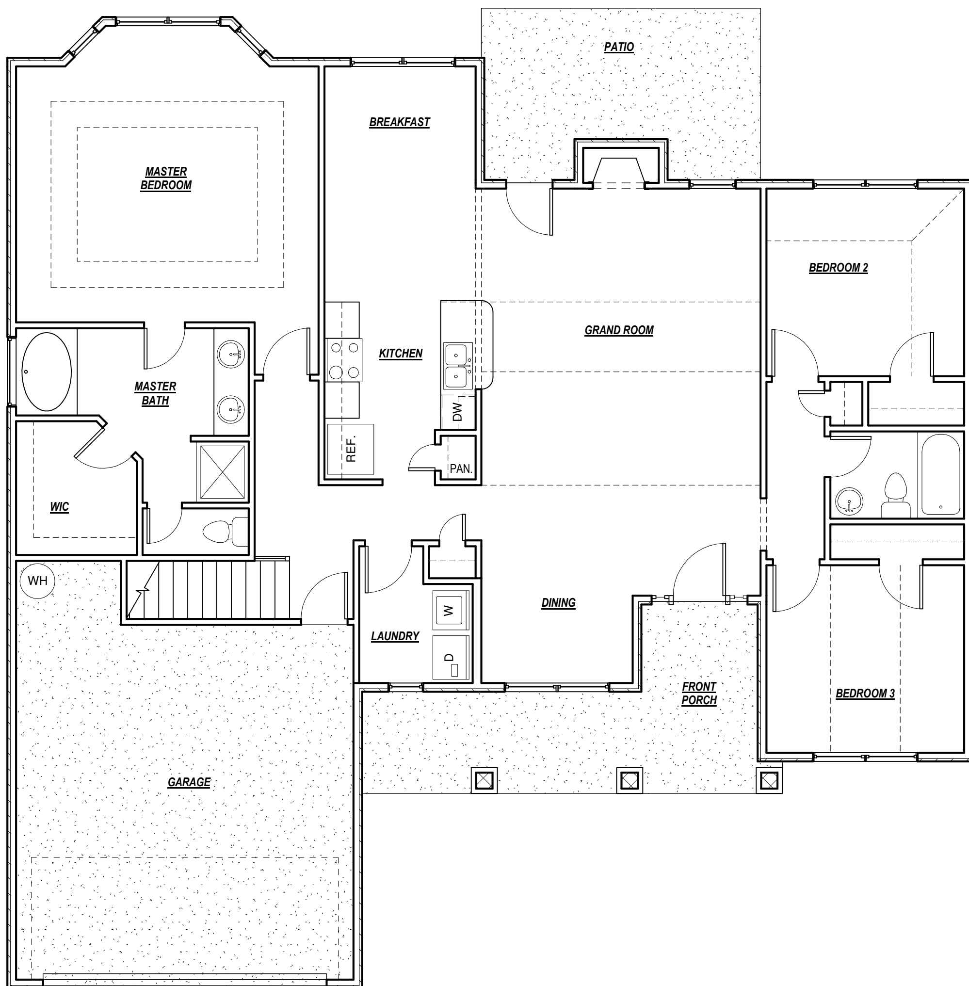
FIRST FLOOR
