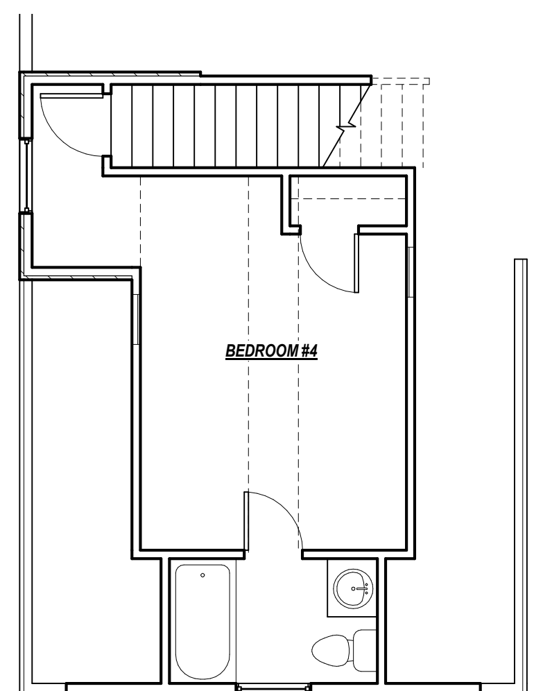
SECOND FLOOR
