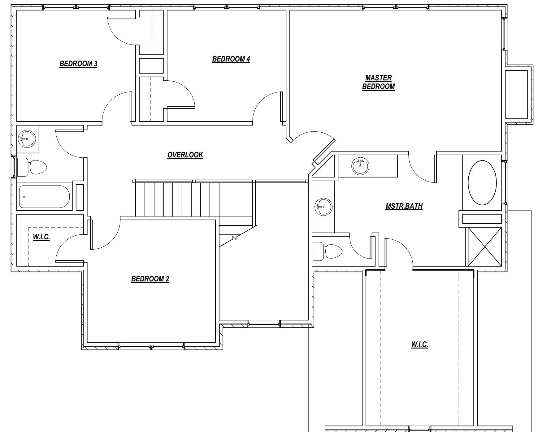
SECOND FLOOR
