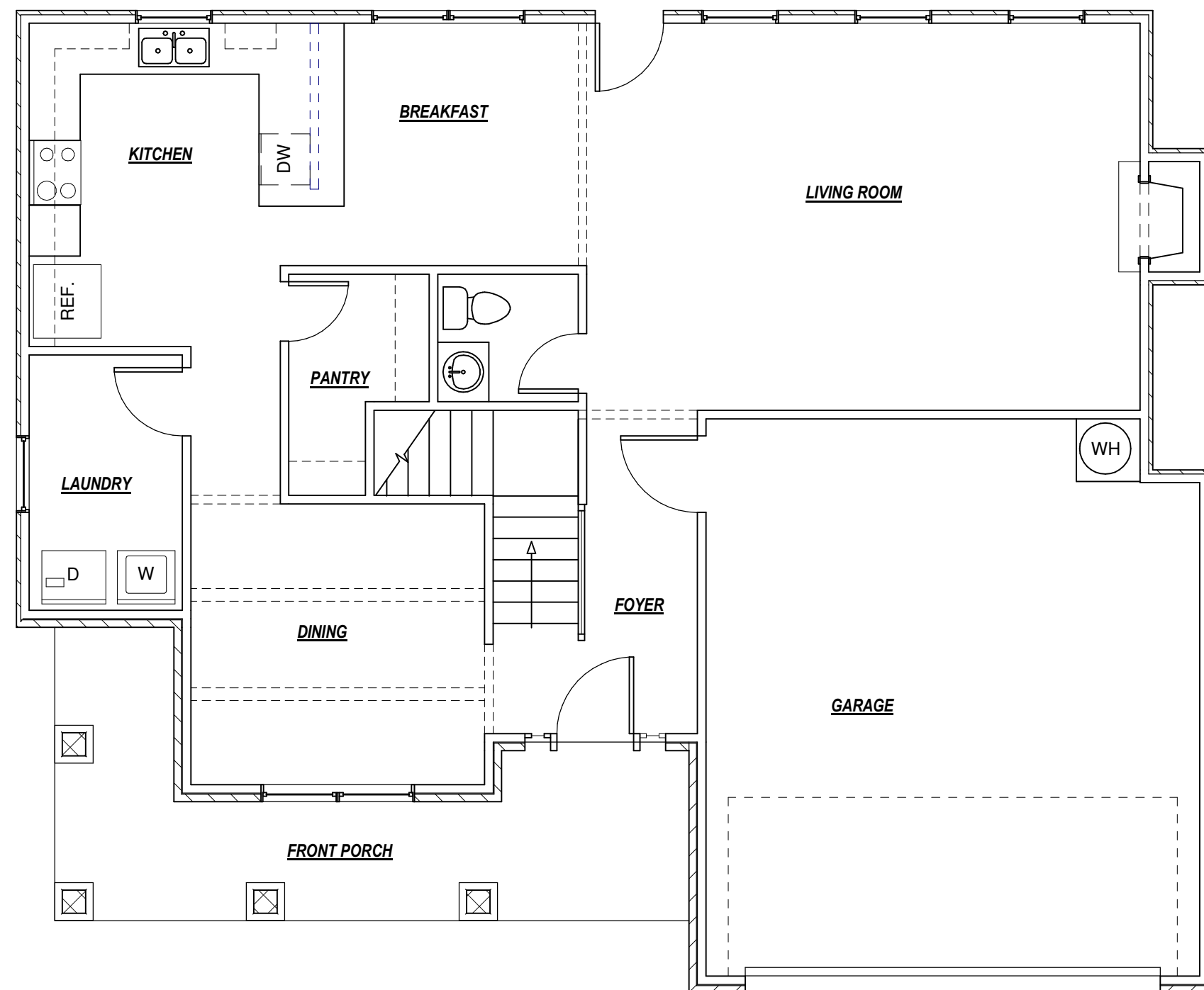
FIRST FLOOR
